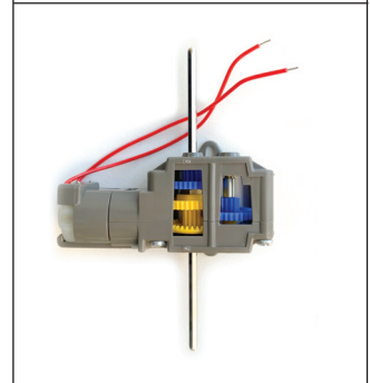
Solar car – Motor and gearbox ST 282-07
